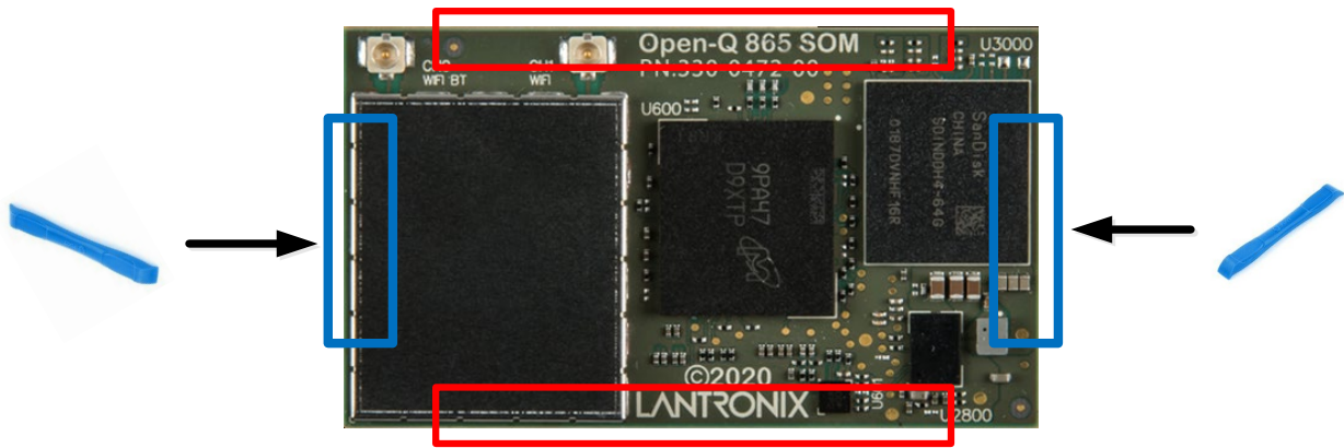
Figure 12: SOM Plastic Prying Tool Removal Locations
