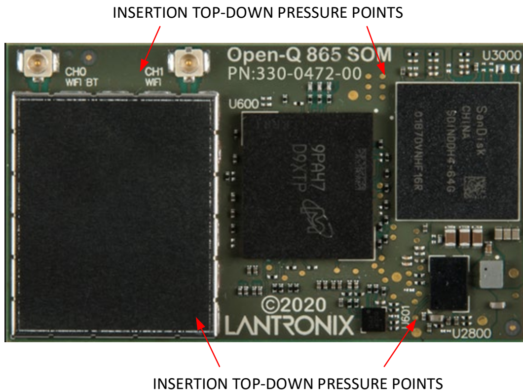
Figure 11: SOM Insertion Top-Down Pressure Locations
